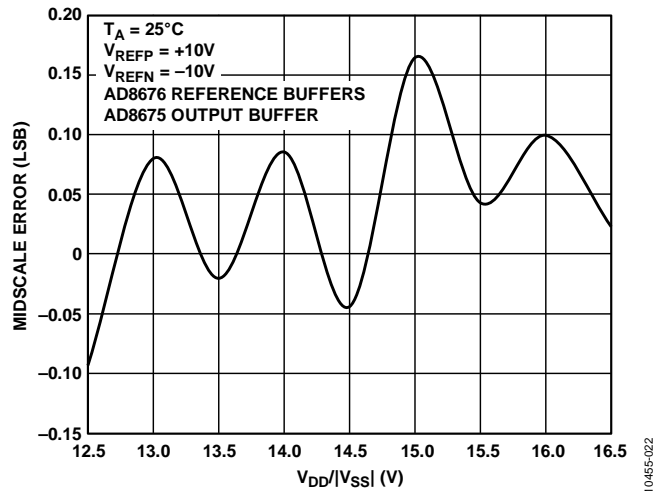
Figure 22. Midscale Error vs. Supply Voltage, ±10 V Span
