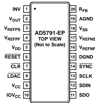
Figure 5. Pin Configuration
