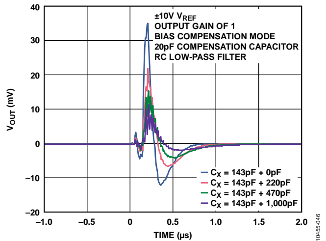
Figure 46. Midscale Peak-to-Peak Glitch for ±10 V
