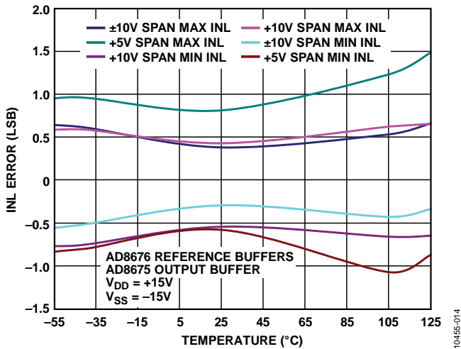
Figure 14. Integral Nonlinearity Error vs. Temperature
